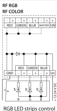
RGB LED strips control
