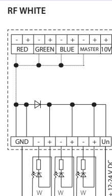
Monochrome LED strips control
